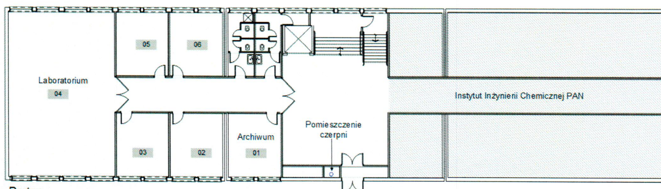
Parter
